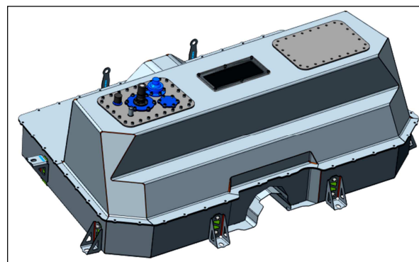
100lts FT3 fuel tank general view
